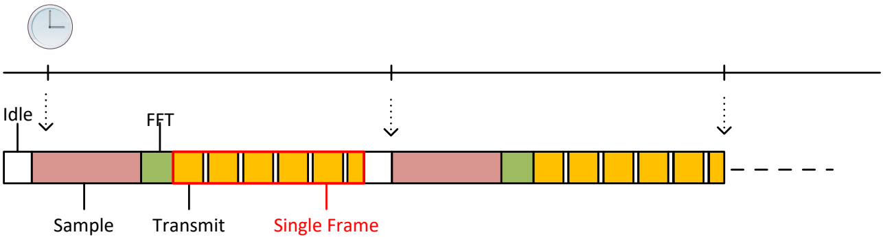
Figure 7: Timing Diagram
