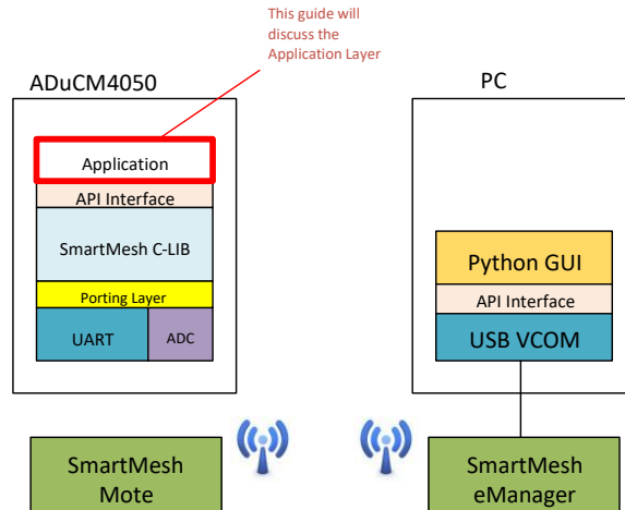
Figure 1: Hardware Overview
