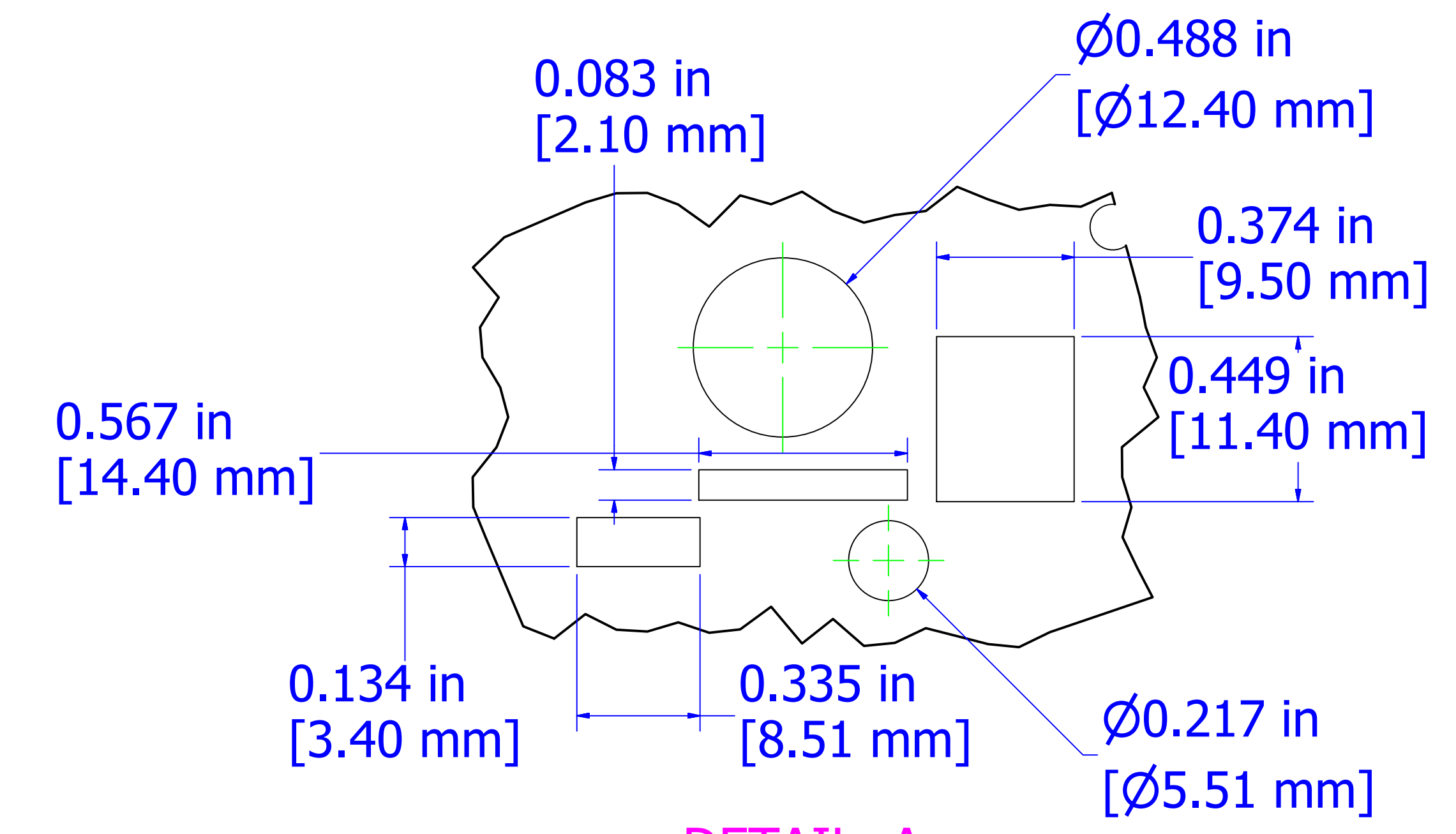
DETAIL A
