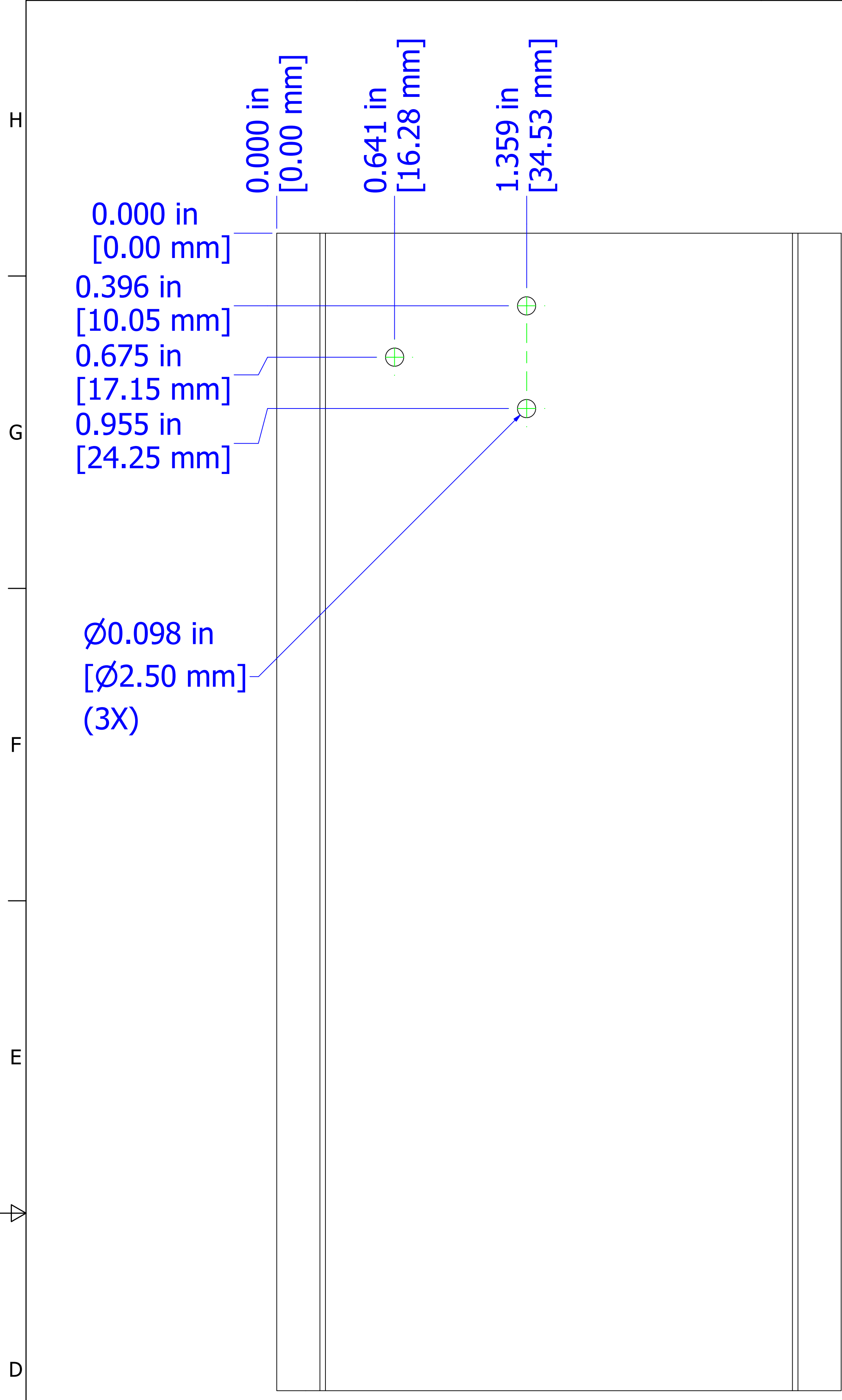
EXTRUSION
