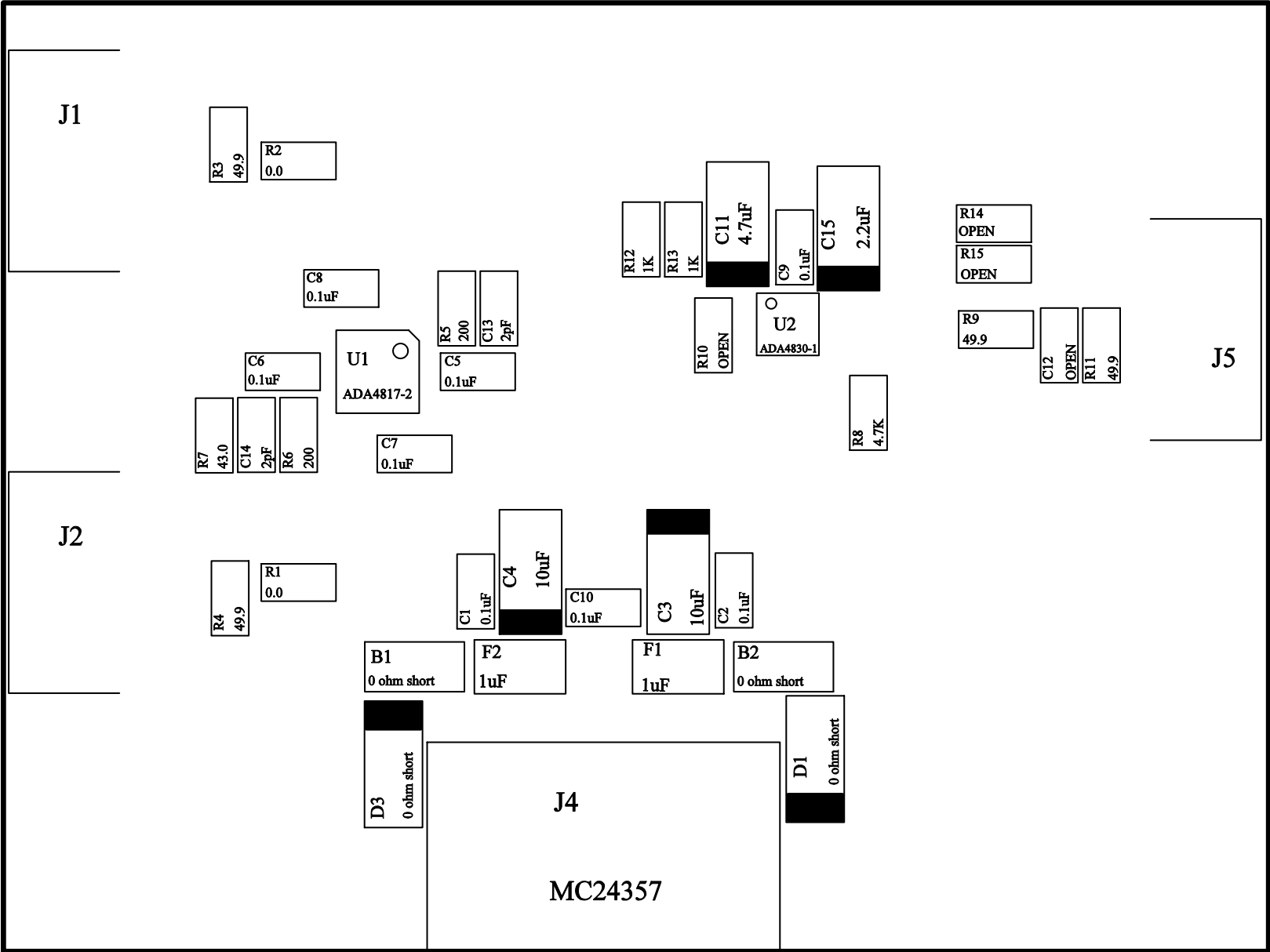
Top Assembly
