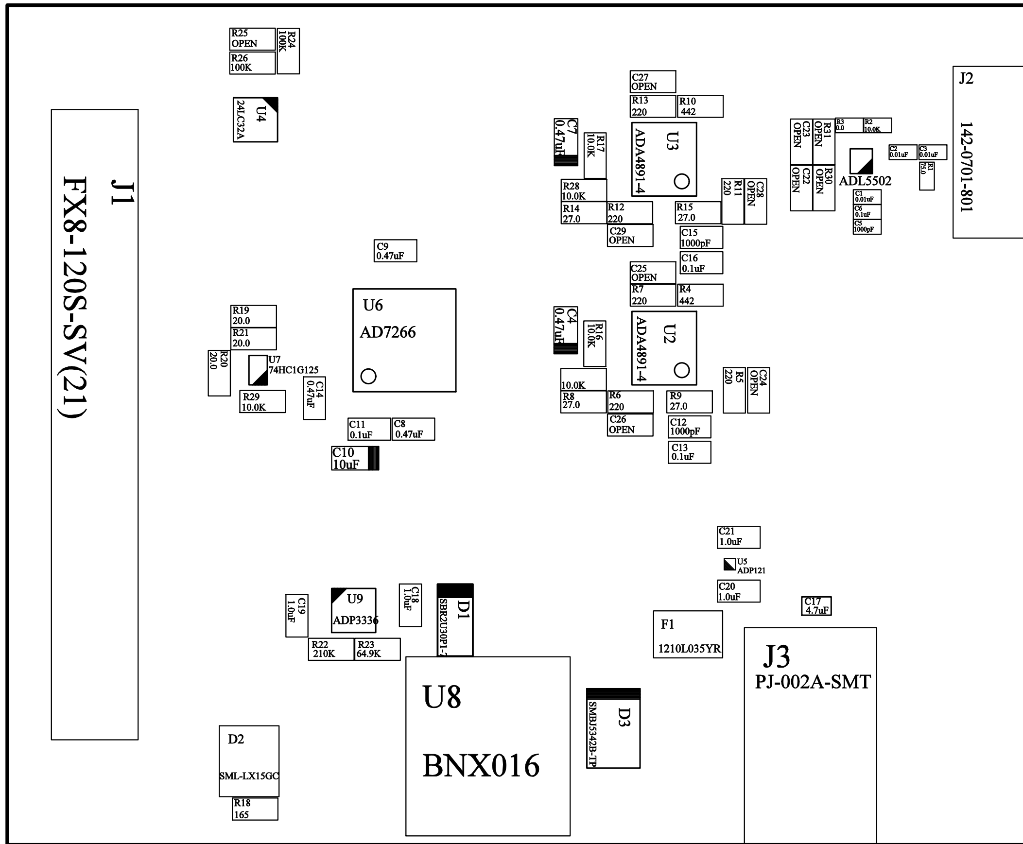
Assembly Top
